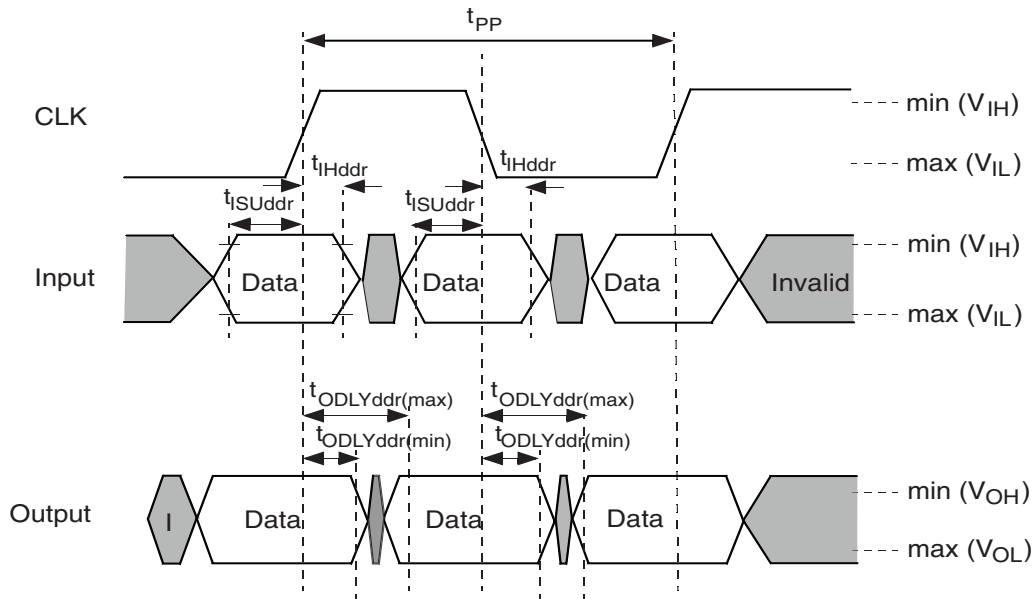
Figure 8. DDR Interface Timing
