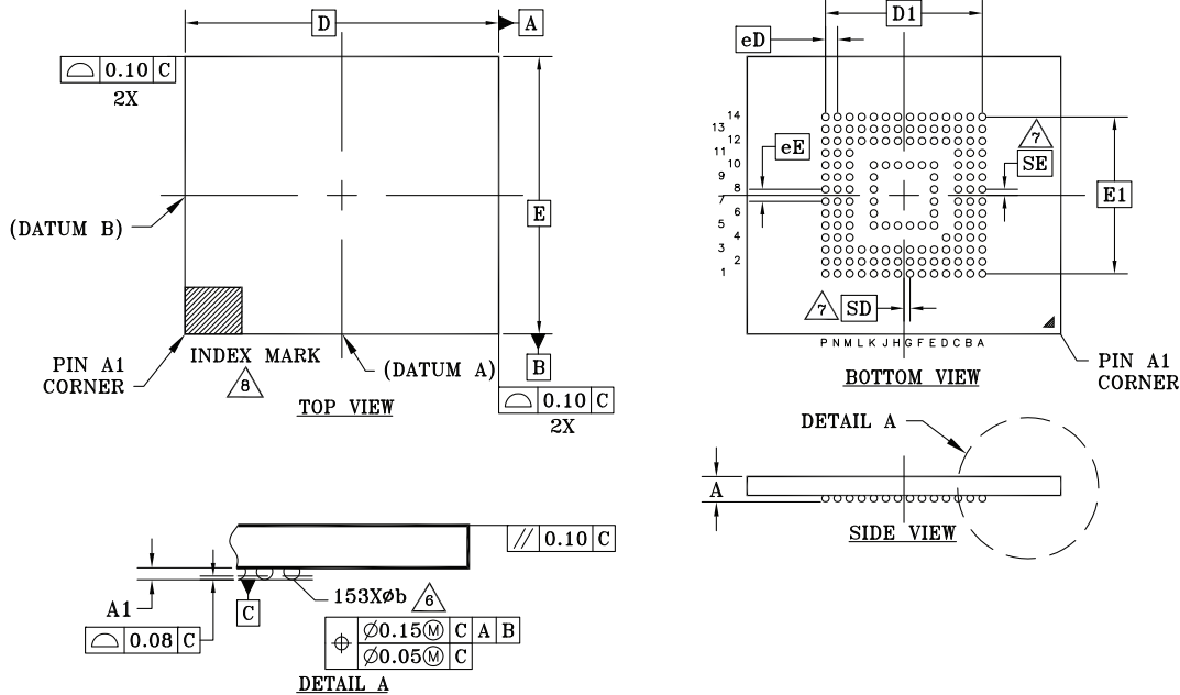
Figure 14. VFBGA 153 (13 × 11.5 × 1.0 mm)
