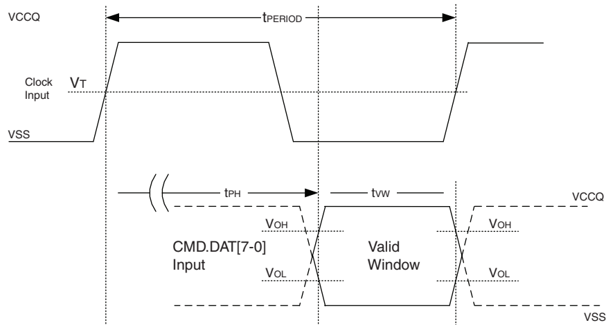
Figure 11. HS200 Device Output Timing [19]
